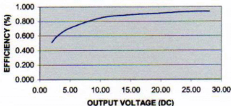
EFFICIENCY VS. Vout
